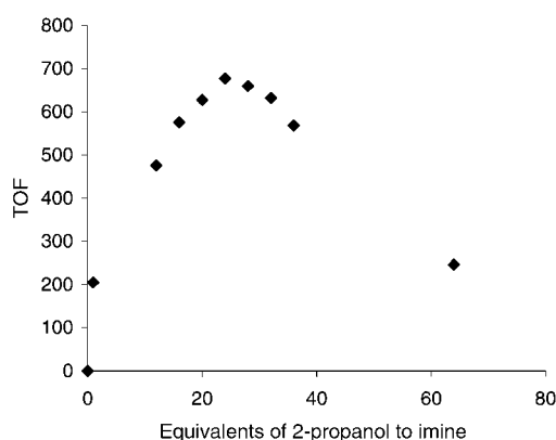
Figure 1. Transfer hydrogenation of 4 according to Equation (2).
