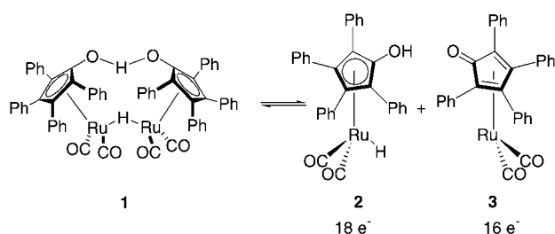
Scheme 2. The dissociation of the dimeric catalyst precursor.
