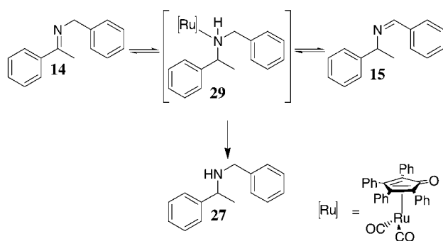
Scheme 4. The isomerization of imine 14 and 15 .
